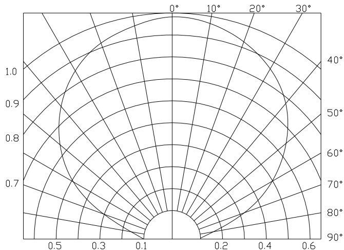
Radiation Diagram
